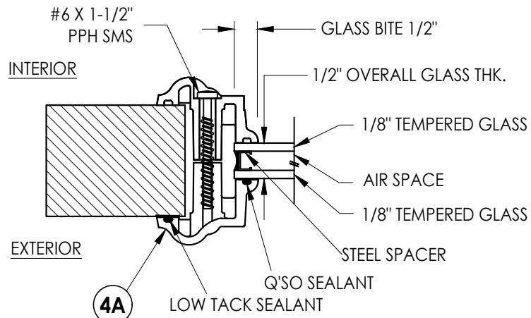
4A GLAZING DETAIL
