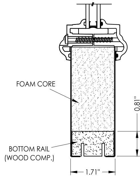
2 4 VERTICAL CROSS SECTION
