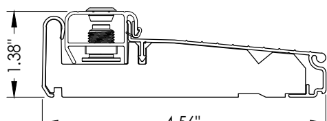
T4 INSWING ADJUSTABLE THRESHOLD ZAIAA4565FN
